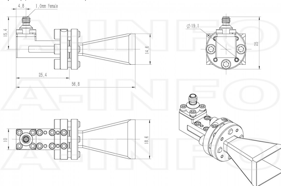
1.0mm-Female Output (P/N: LB-12-20-C-1.0F)
